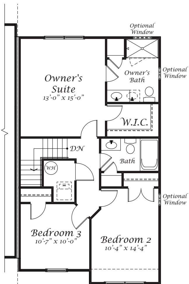
Three Bedroom Option
