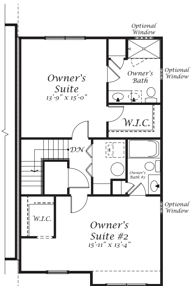
Double Master Option
