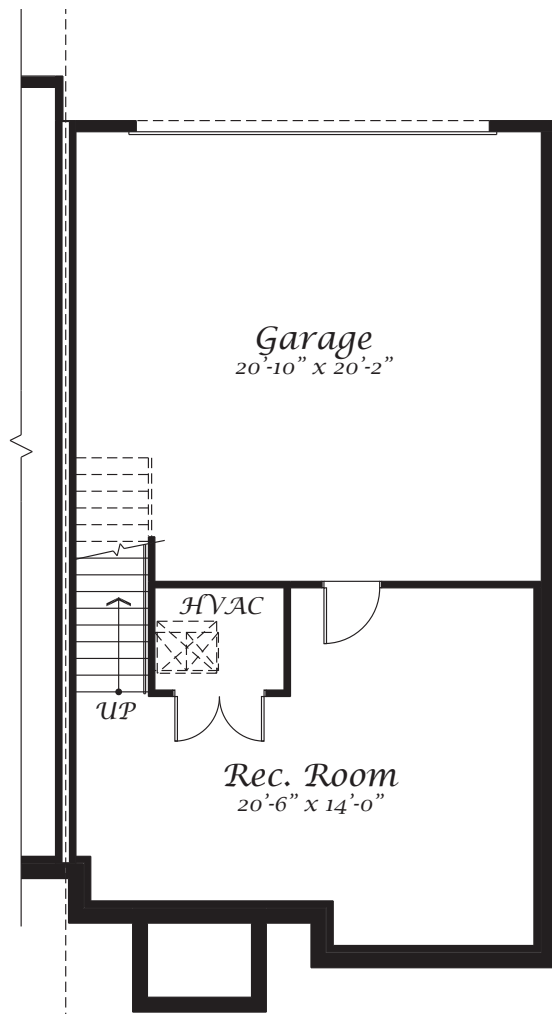
Optional Two Car Garage
