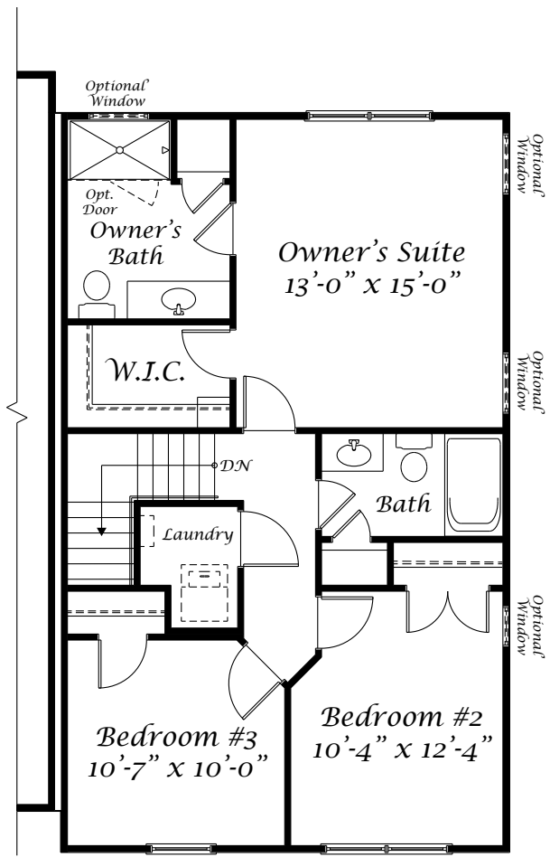
Three Bedroom Option
